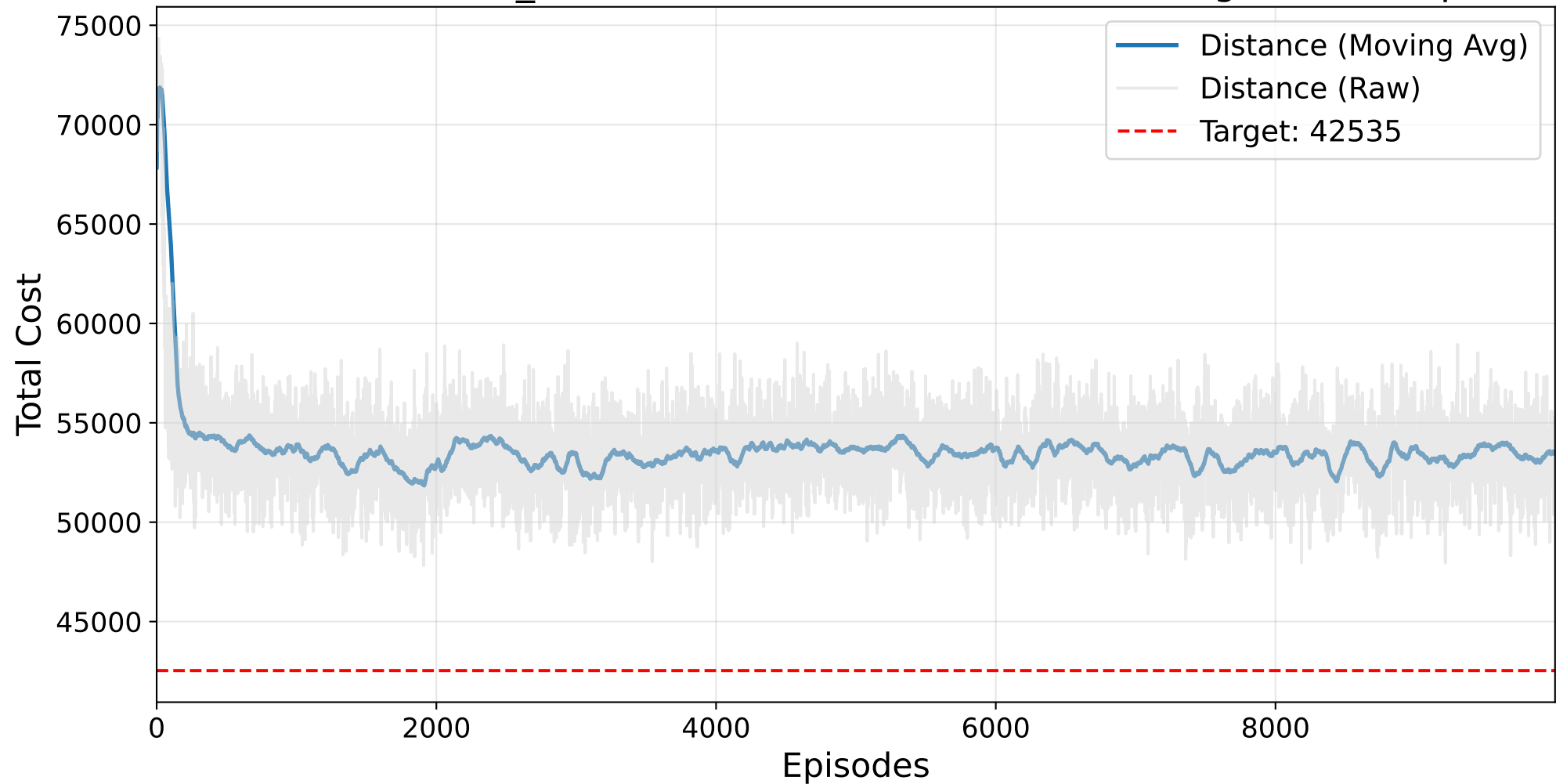
Final RANDOM_SEARCH Masked AutoRL-SOP Training - ft70.3.sop
